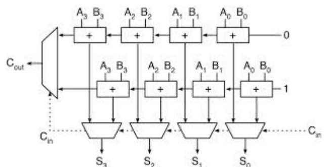
Fig. 2 Carry Select Adder
