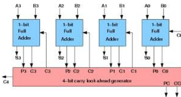
Fig. 5 Carry Increment Adder
