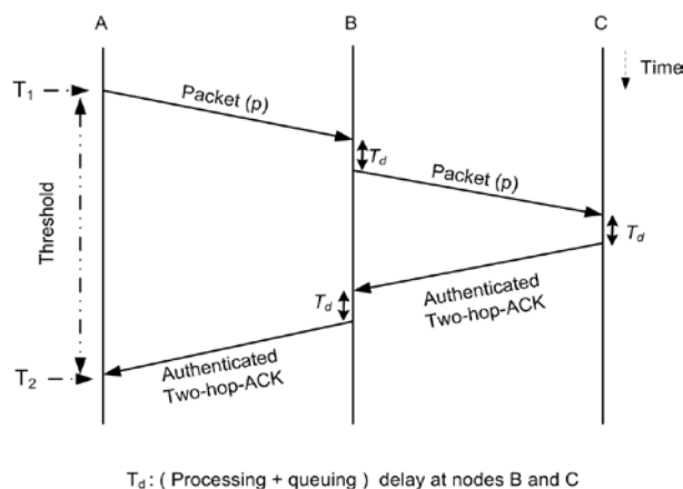
Figure 4.1 Ack-Based Approaches
