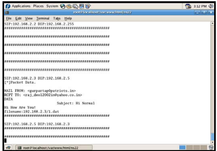
Figure 4. Spam capture program displaying a normal mail
