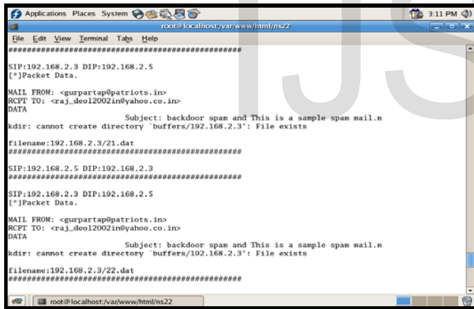
Figure 3. Spam capture program displaying a spam mail
