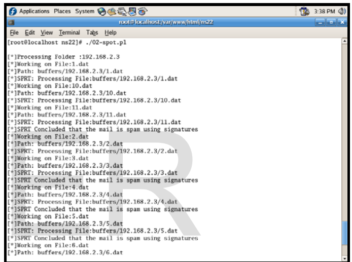
Figure 5. Spam capture program displaying a spam mail
