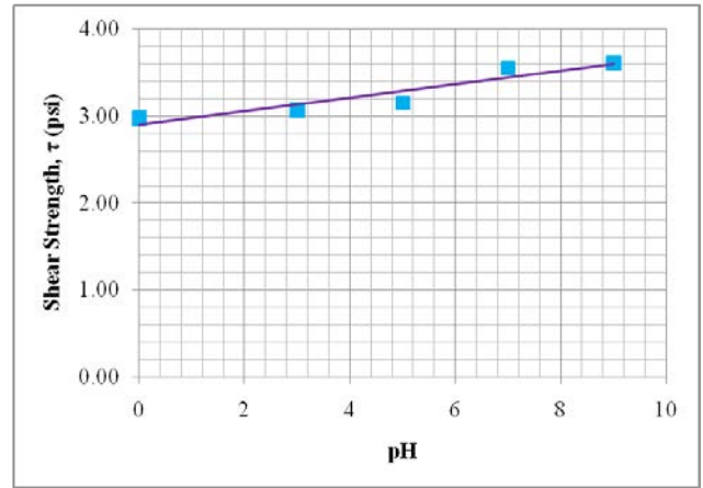
Fig.1 Shear strength Vs. pH values of S -1.
