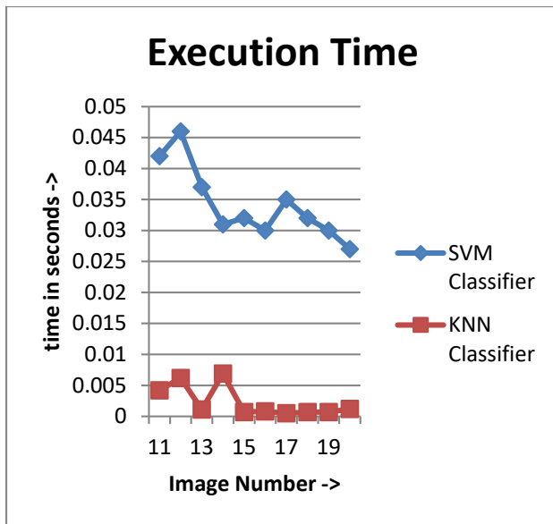
Fig 3: Execution Time
