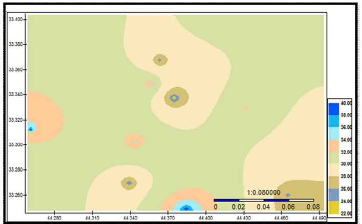
Fig.5. Spatial distribution map of Ni metal in Baghdad gardens soil.
