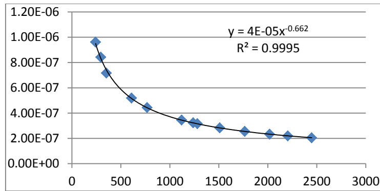
Figure.2 The absolute energy peak efficiency measurement using the standard sources 226 Ra and 60 Co
