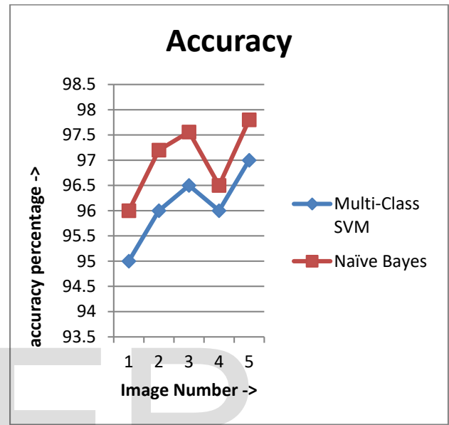
Fig 2: Accuracy Comparison
